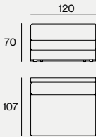
ELEMENT D 120X107X70H
