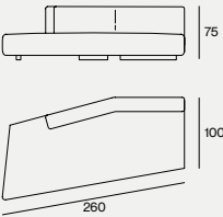
SOFA ELEMENT H LH 260X100X75H
