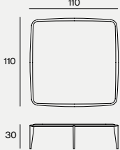
DIMENSIONS 110X110X30H
