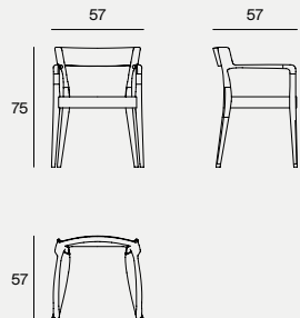
DIMENSIONS 57X57X75H
