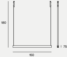
DIMENSIONS 150X7.5H
