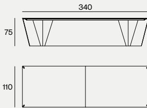
DIMENSIONS 340X110X75H
