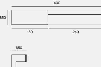
DIMENSIONS 400X65X55H
