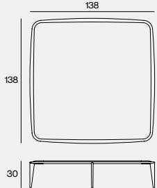
DIMENSIONS 138X138X30H
