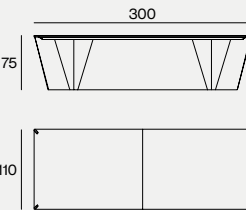
DIMENSIONS 300X110X75H
