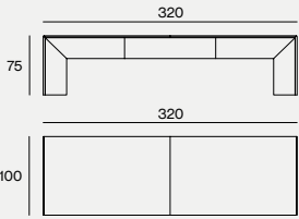
DIMENSIONS 320X100X75H
