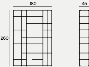
DIMENSIONS 180X45X260H
