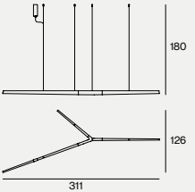
DIMENSIONS 311X126X8H - XL C
